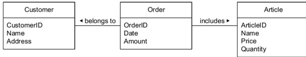
Fig. 1.6: A data model for customers, orders, and articles
